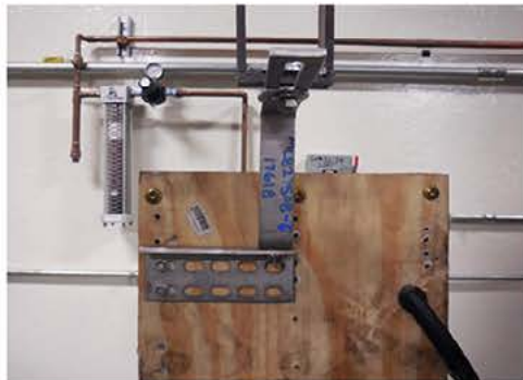
Photo 9: Shear Test Setup
